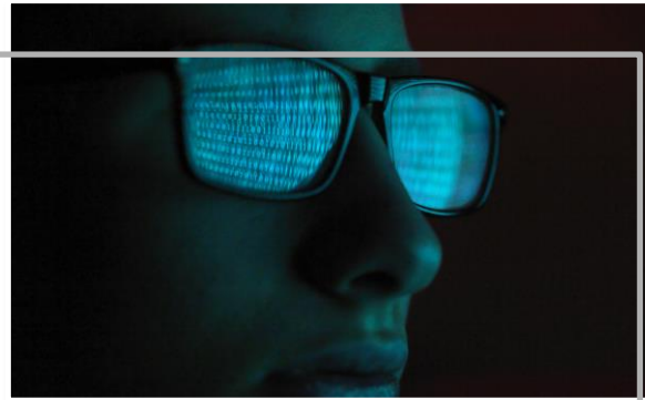
OT/IOT Cybersecurity
